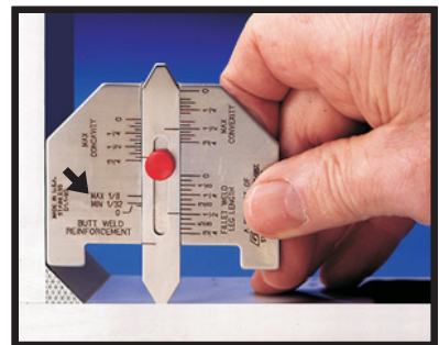
TO DETERMINE THE LEG SIZE OF THE FILLET WELD
