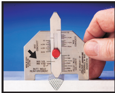
CHECK REINFORCEMENT
